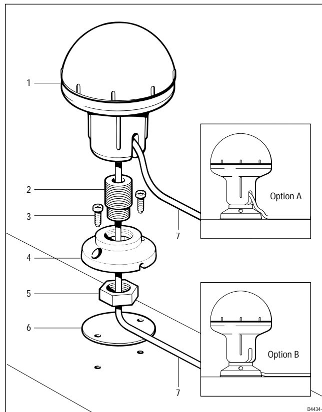
1 Sensor 2 Threaded connector 3 Screws 4 Retaining ring 5 Nut 6 Seal 7 Cable
