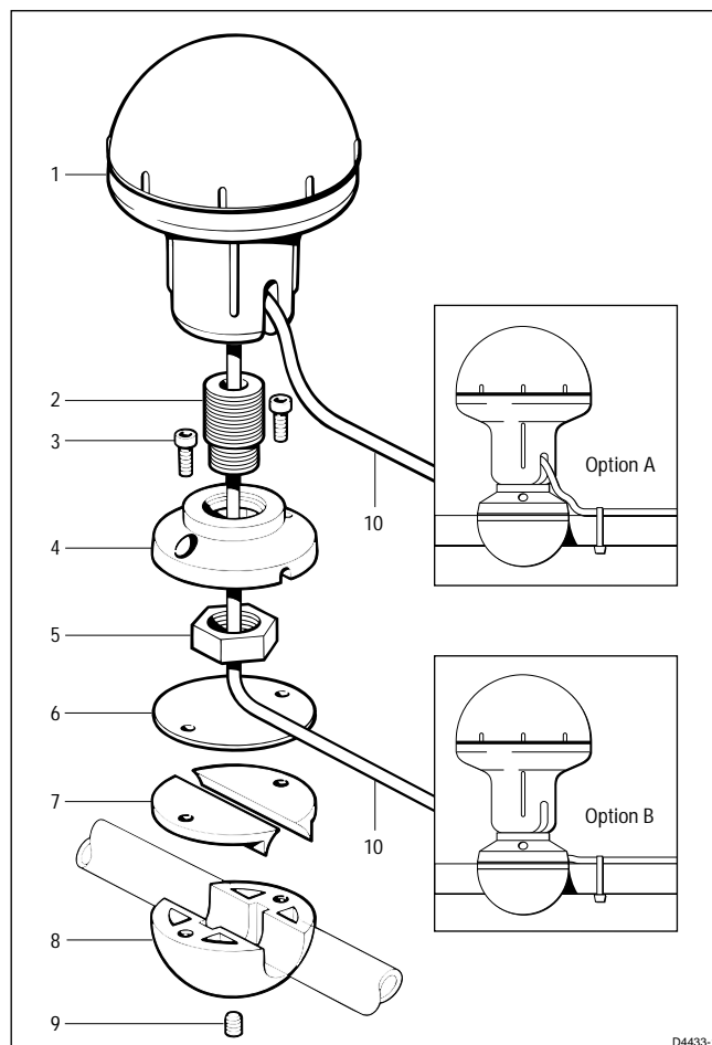
1 Sensor 2 Threaded connector 3 Bolts 4 Retaining ring 5 Nut 6 Seal 7 Spacers 8 Rail Clamp 9 Grub screw 10 Cable
