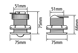
ST40 Speed and Depth Transducer Dimensions
