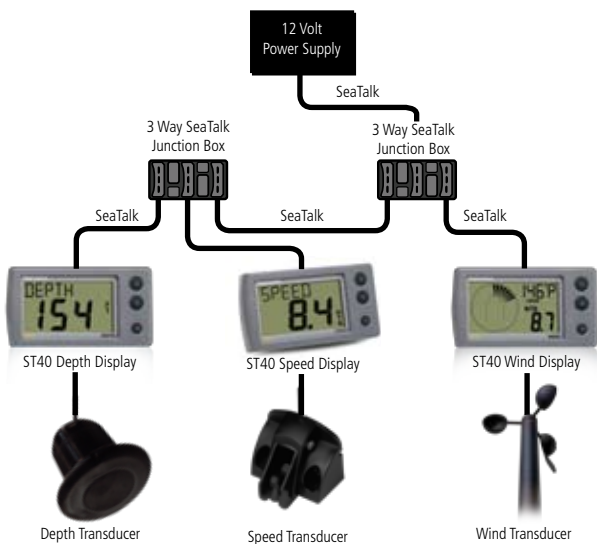
Typical ST40 Depth, Speed and Wind System
