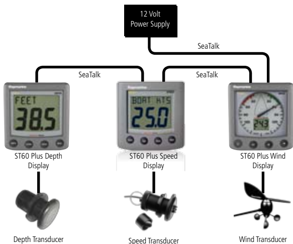
Typical ST60 Plus Depth, Speed and Wind System
